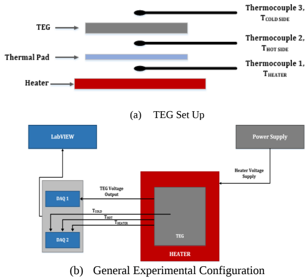
Figure 1: Schematic representation of experimental facility
