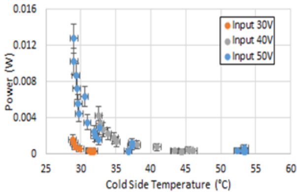
Figure 4: Power Output vs. Cold Side Temp. for No Cooling
