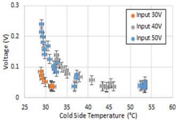
Figure 3: Voltage Output vs. Cold Side Temp. for No Cooling
