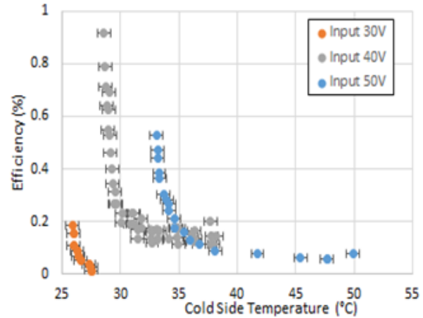
Figure 5: Efficiency vs. Cold Side Temp. for Fin Cooling
