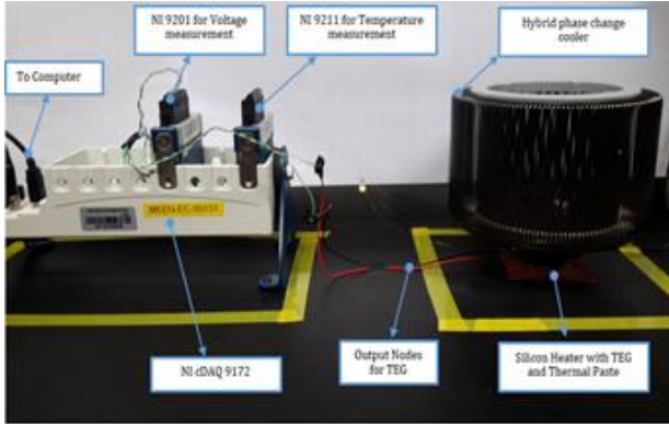
Figure 2: Experimental Setup for Hybrid Cooling Method
