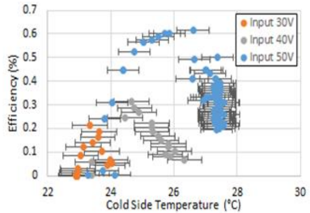
Figure 6: Output Efficiency vs. Cold Side Temperature for Hybrid Cooling
